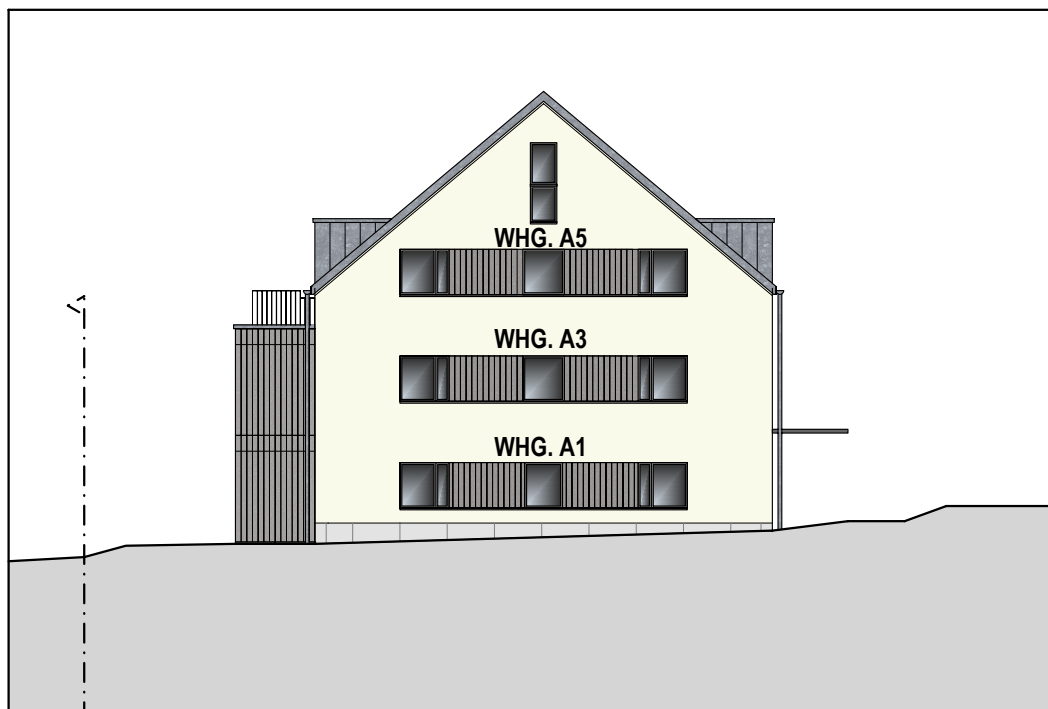
MFH A OST-FASSADE
